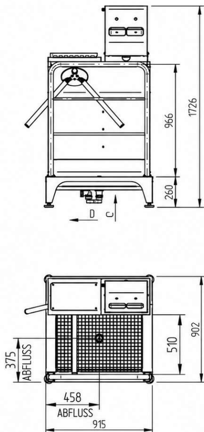
1227101040 DSO 01B.1P.915
